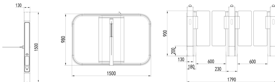
LA3220-B-R/L Single Channel
