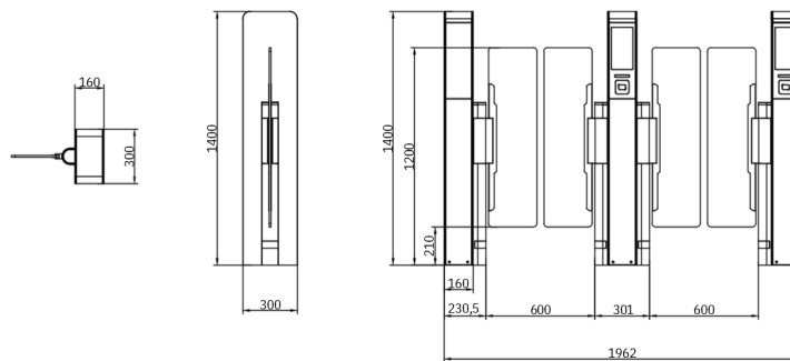
LA3219H-R/L/M Two Channel
