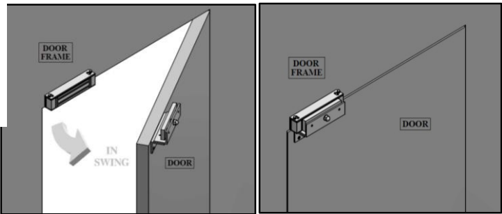
Installation Diagram
