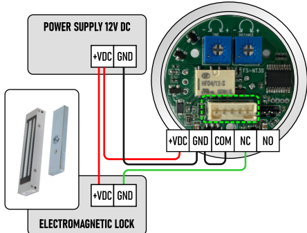
Fail-Safe Lock
