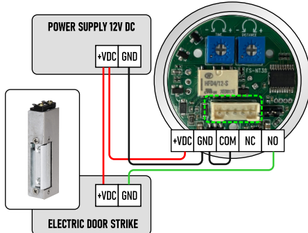
Fail-Secure Lock
