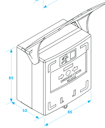
Line drawing with 30mm back box
